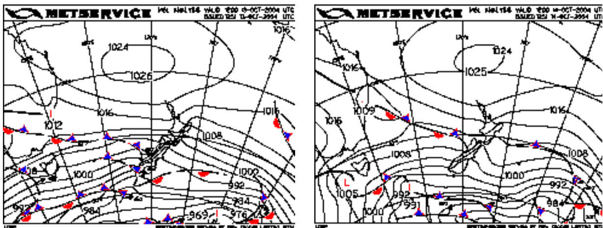
Figure 11: Synoptic weather charts for New Zealand on 13 th (left) and 14 th (right) October 2004.
